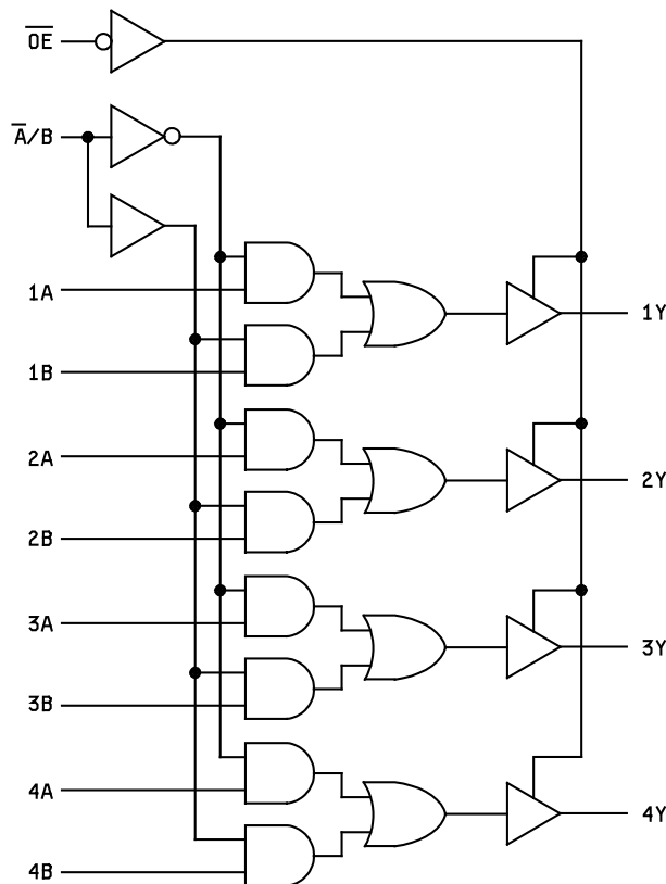
FIGURE 3. Logic diagram.
