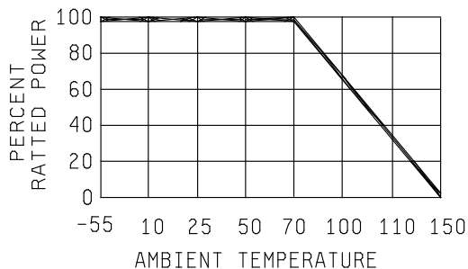
FIGURE 2. Derating curve .
