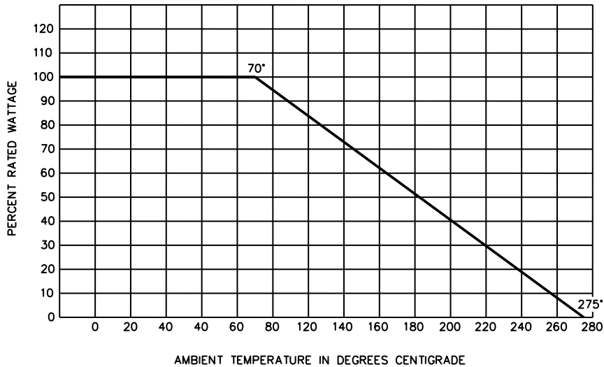
FIGURE 2. Derating curves for high ambient temperatures.
