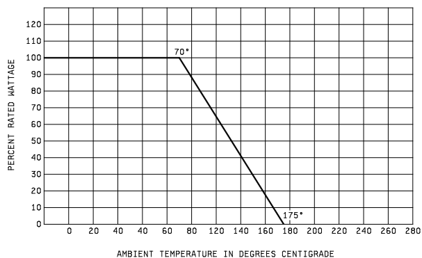
FIGURE 2. Derating curves for high ambient temperatures.
