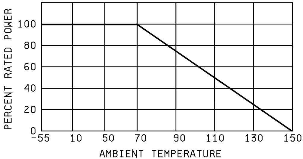
FIGURE 2. Derating curve .
