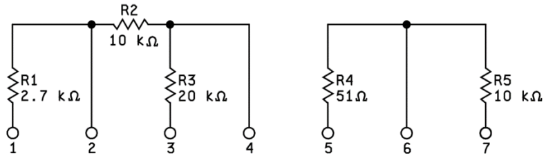
SCHEMATIC - 04
