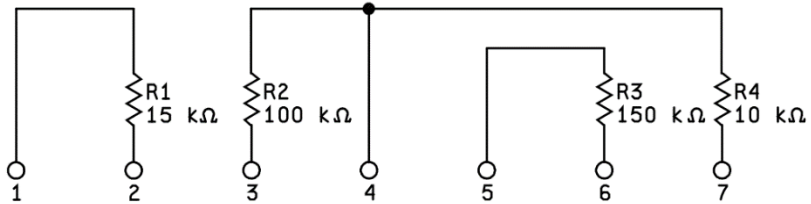
SCHEMATIC - 05
