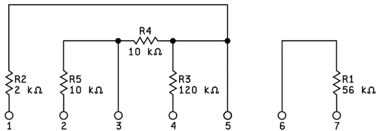
SCHEMATIC - 06
