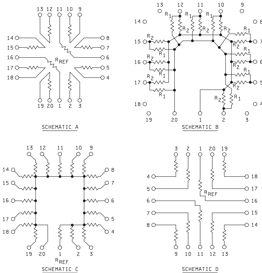
FIGURE 1. Schematics .
