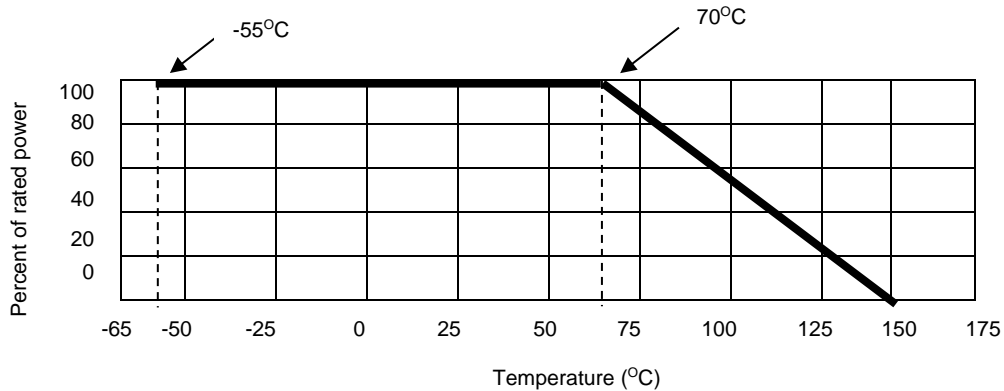
FIGURE 2. Derating curve.
