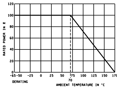
FIGURE 2. Derating curves for high ambient temperatures.
