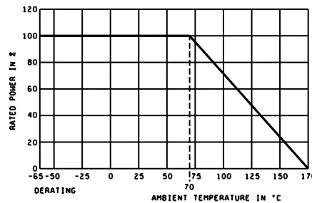
FIGURE 2. Derating curves for high ambient temperatures .
