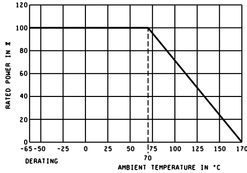
FIGURE 2. Derating curves for high ambient temperatures.
