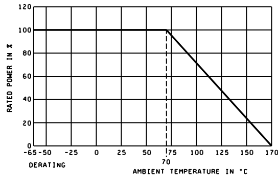
FIGURE 2. Derating curves for high ambient temperatures.
