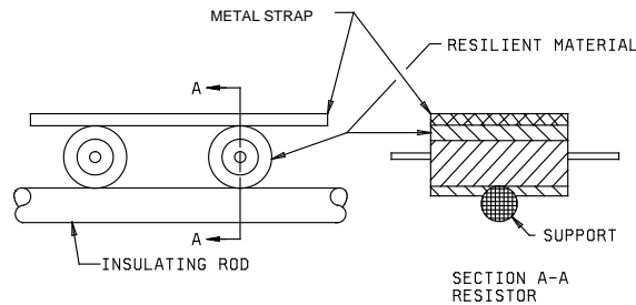
FIGURE 3. Resistor-contacting assembly for dielectric strength.
