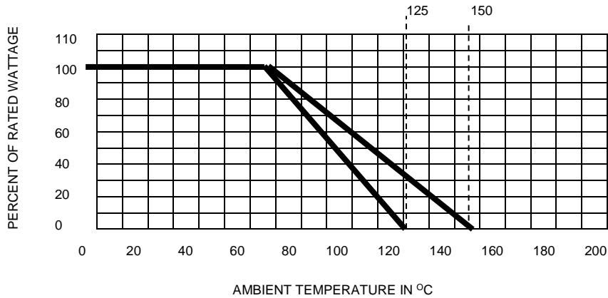
FIGURE 2. Derating curve for high ambient temperatures.
