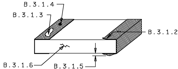
FIGURE B-1. Conductor metallization defects.
