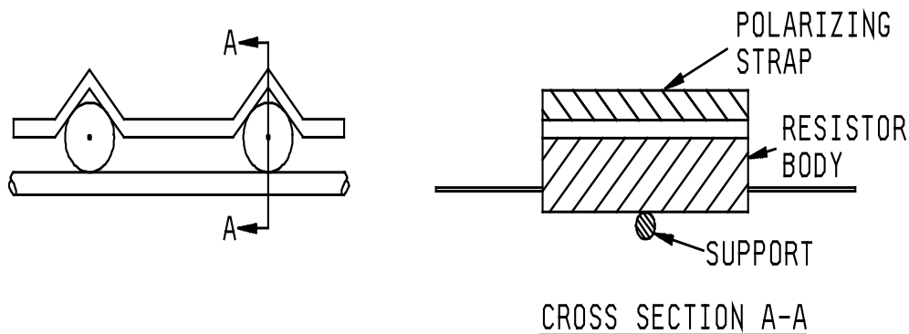
FIGURE 2. Mounting straps for moisture-resistance test.
