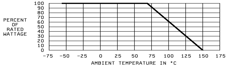
FIGURE 1. Derating curve for high ambient temperatures.
