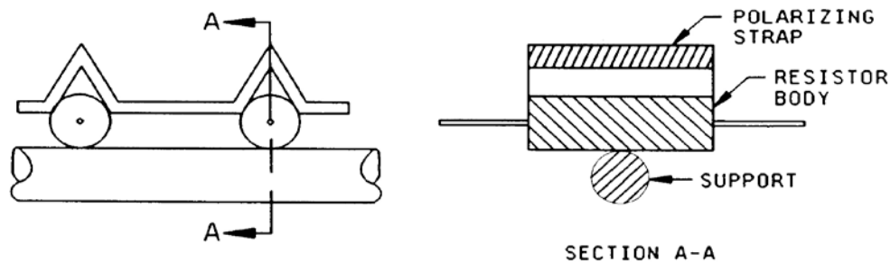
FIGURE 2. Mounting straps for moisture-resistance test for polarized units only.
