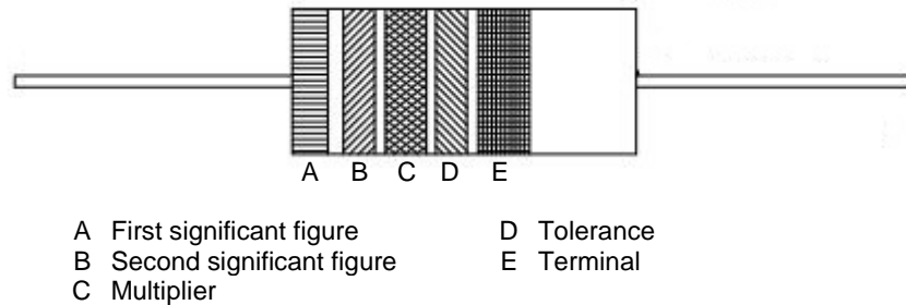
FIGURE B-1. Color-code marking for film-type resistors.
