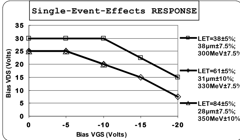
FIGURE 5. SEE safe operating area graph (2N7478T1).
