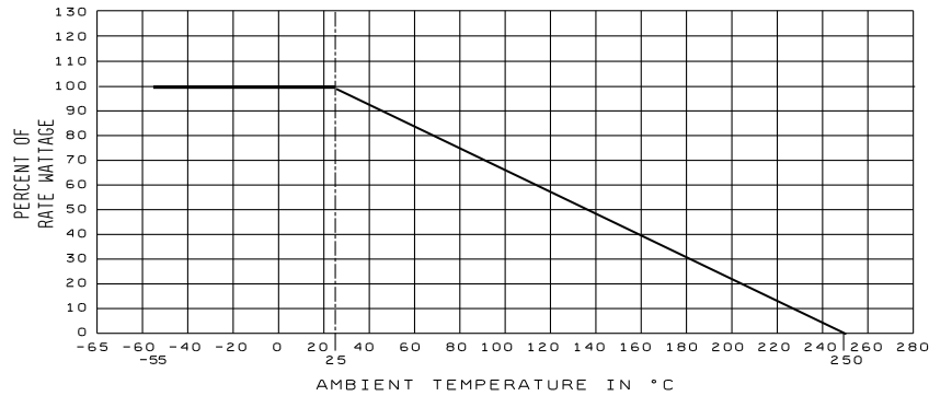
* FIGURE 1. Derating curves for high ambient temperatures.
