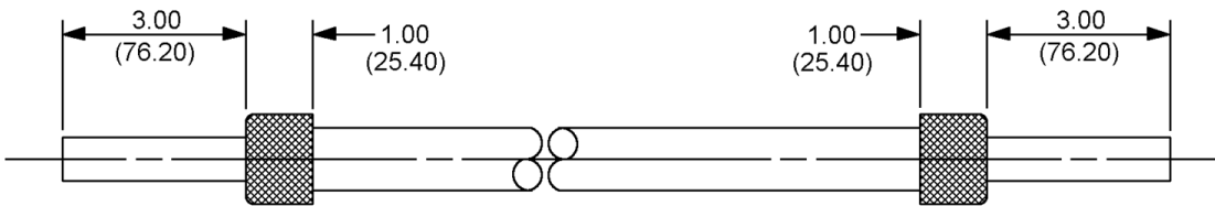
FIGURE 15. Suggested method for making cable ends corona free.
